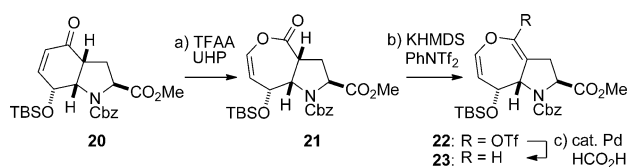
Scheme 3. Synthesis of dihydrooxepine 23 . Reagents and conditions: a) TFAA, UHP, \text{CH}_2\text{Cl}_2 , -20^\circ\text{C} , 53% total yield after 4 reaction cycles (19% of 20 recovered; after a single reaction cycle: 23% yield, 65% yield based on recovered starting material); b) KHMDS, PhNTf 2 , THF, -78^\circ\text{C} ; c) cat. Pd(OAc) 2 , PPh 3 , HCO 2 H, n\text{Bu}_3\text{N} , DMF, 65^\circ\text{C} , 94%. DMF = N,N -dimethylformamide, KHMDS = potassium hexamethyldisilazide, TFAA = trifluoroacetic anhydride, UHP = urea hydrogen peroxide.
